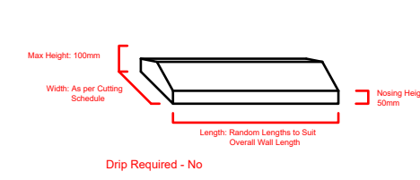
Twice Weathered Coping - Straight Stone Reference: CO...
