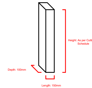
Plain Jamb/Mullion - Square Section Stone Reference: Jamb - J... Mullion - M...
