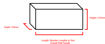
Plain Plinth - Square Section Stone Reference: P...
