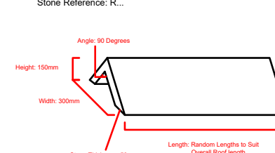
Angled Ridge Stone Reference: R...
