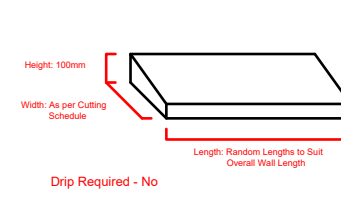
Once Weathered Coping - Straight Stone Reference: CO...
