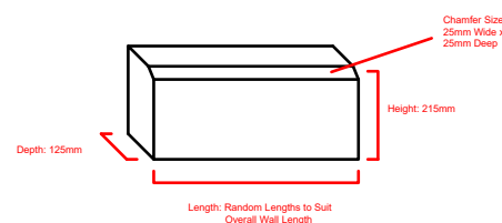
Chamfered Plinth - Straight Stone Reference: P...
