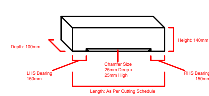
Chamfered Head Stone Reference: L...
