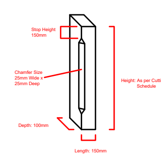
Chamfered Jamb Stone Reference: J...
