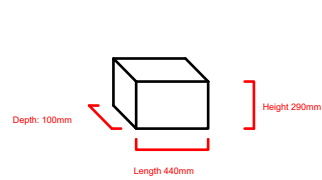
Plain Quoin - Square Section Stone Reference: Q...
