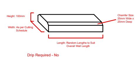
Chamfered Coping - Straight Stone Reference: CO...
