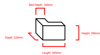
L Shaped Quoin - Square Section Stone Reference: Q...
