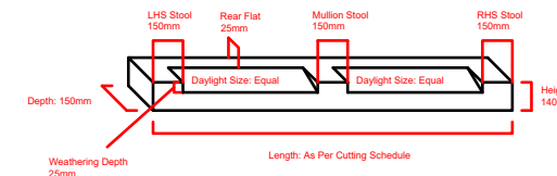
Stooled Cill - Mullion Window Stone Reference: C...
