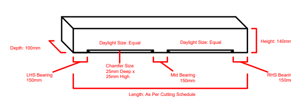
Chamfered Head - Two Light Window Stone Reference: L...
