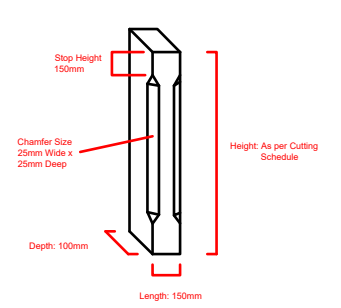
Chamfered Mullion Stone Reference: M...
