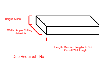
Flat Coping - Square Section Stone Reference: CO...
